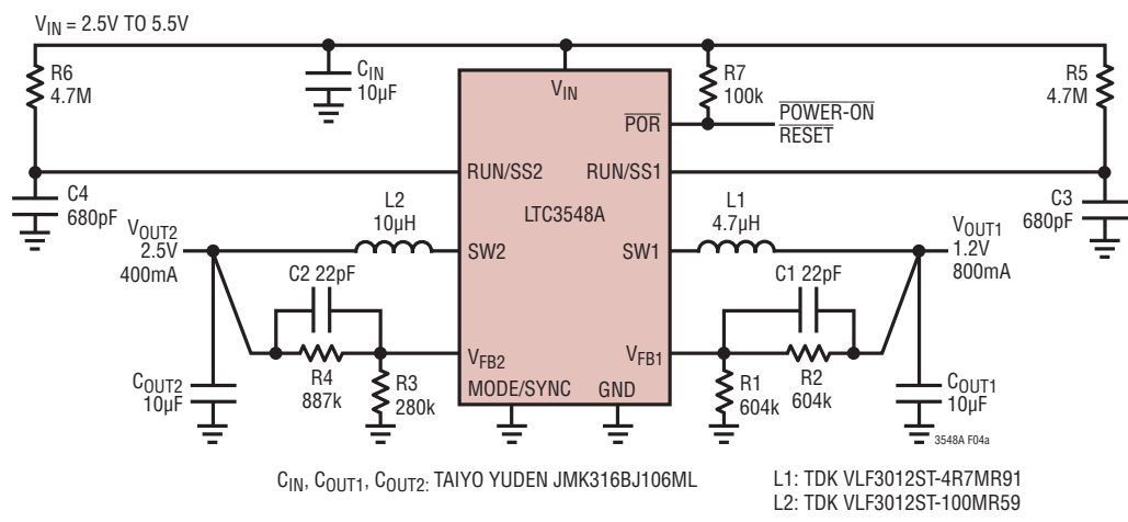
Figure 4. Low Ripple Buck Regulators with Soft-Start
